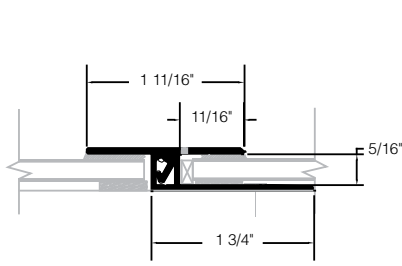
Two Piece Divider MIN-66 receptor & MIN-69 divider
