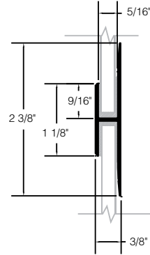
One Piece Divider MIN-40
