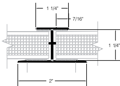
One Piece Divider MW-22943
