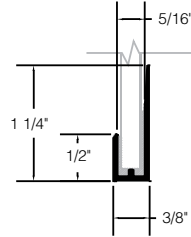
One Piece Cap MIN-39
