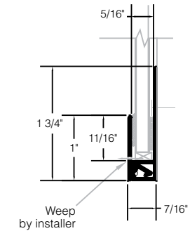
Two Piece Cap MIN-66 receptor & MIN-67 cap
