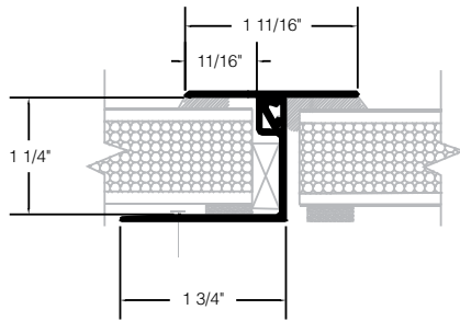
Two Piece Divider MIN-68 receptor & MIN-69 divider
