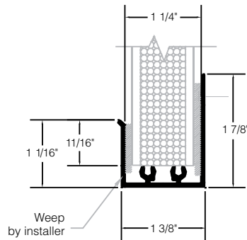
One Piece Cap MW-22944
