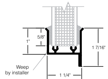
Add-on / Projected Sash MW-16610
